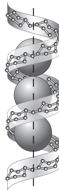
iodine atoms in a linear pattern within the coils of a starch molecule
